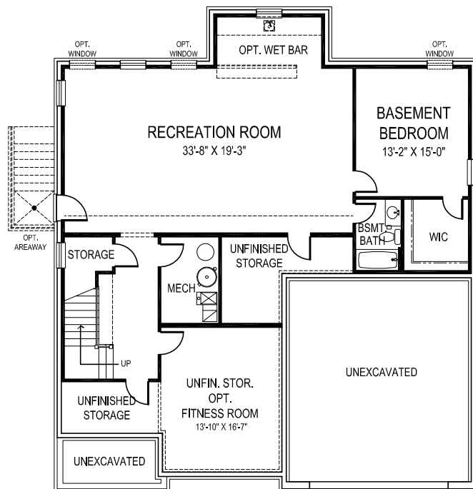
BASEMENT PLAN
