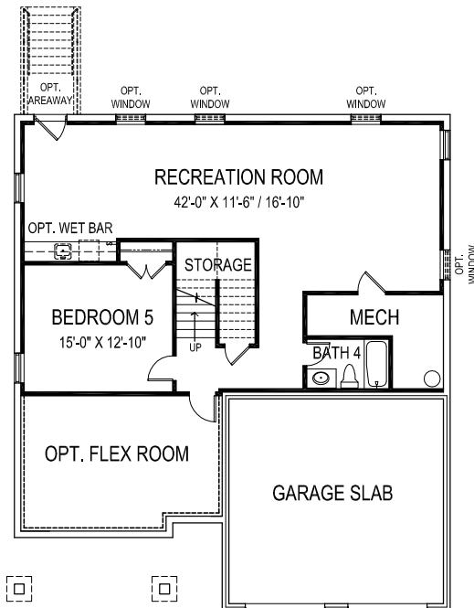
BASEMENT PLAN
